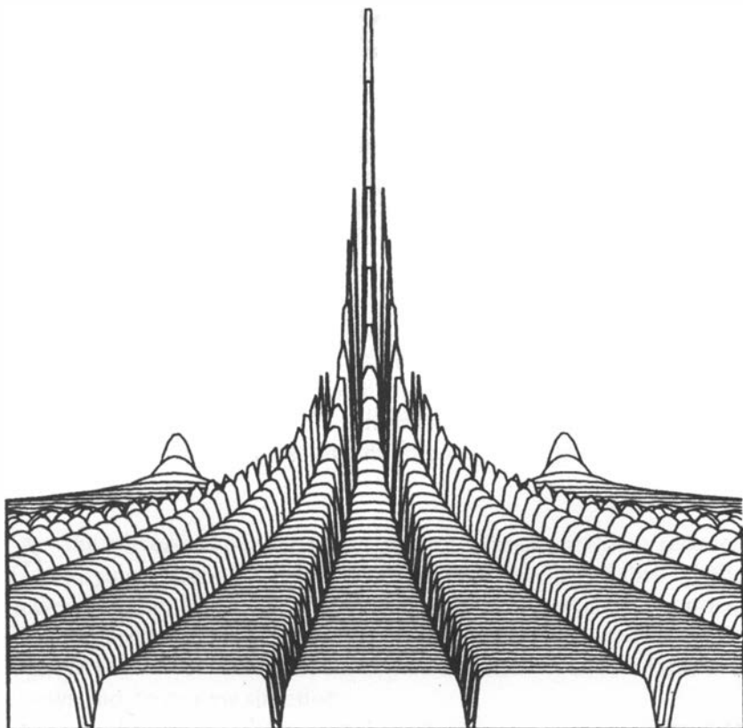
Figure 11. Bohm's quantum potential. This curved surface represents Bohm's quantum potential for the case of an electron passing through two slits. The potential surface guides the electron so that it moves in a manner consistent with quantum mechanics.
