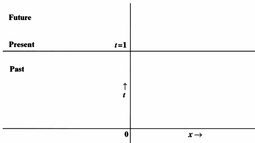
Figure 6. Diagram of past, present, and future. In classical physics, space is static and time is dynamic. Here three-dimensional space is represented by the x -axis for simplicity. Time is represented by the t -axis. The “present” at time t=1 is marked by a horizontal line, with the past below it and the future above it.
