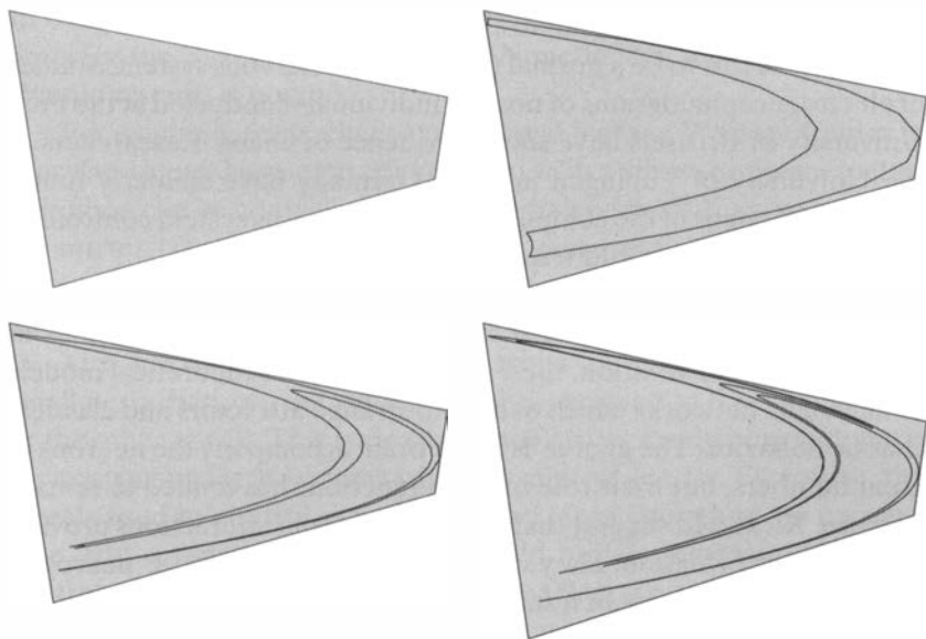
Figure 5. The Henon strange attractor. M. Henon (1976) described a simple transformation that takes the shaded quadrilateral (top left), stretches it, bends it into a U-shape, and puts it back into the quadrilateral. When this operation is repeated, the U is stretched and bent into a double U inside the U, a quadruple U inside the double U, and so on. In the limit, this becomes an oddly shaped set called a strange attractor. Due to the stretching, two points that initially are close together in the shaded quadrilateral will be sent to completely different locations on the strange attractor. This is a simple example of the kind of exponential amplification that occurs in more complicated situations in the real world.
